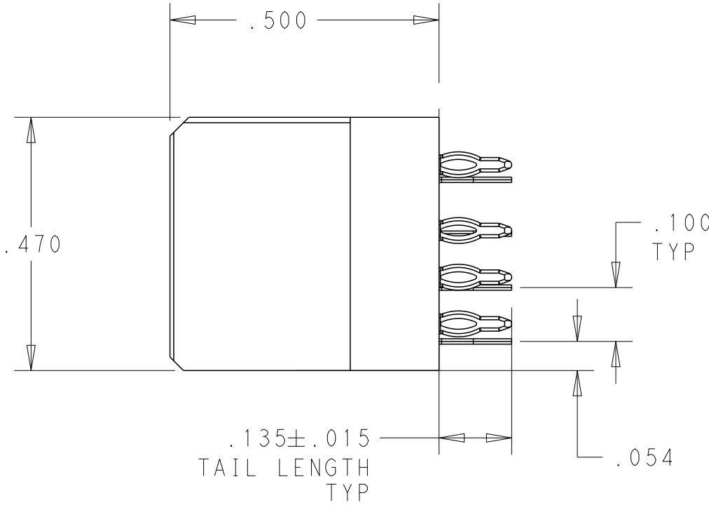
SIGNAL PINS SIDE VIEW
